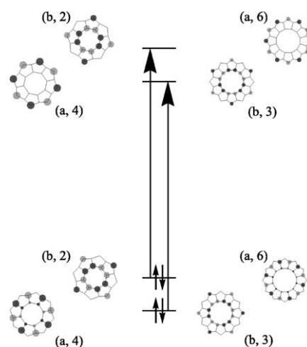
Figure 3. Virtual excitations between frontier orbitals that produce the paratropic ring currents in [8,5]- and [12,5]coronenes. Each orbital is labeled ( \Gamma, A ) with symmetry \Gamma (a or b) and angular momentum A . In each case, there is a rotationally allowed [(\Gamma, A) \rightarrow (\Gamma, A)] excitation from HOMO–1 to LUMO and from HOMO to LUMO + 1. The distribution of coefficients shows that the inner current arises from the HOMO in [8,5]- but HOMO–1 in [12,5]coronene, and vice versa for the outer current.
